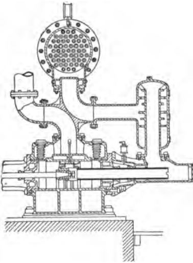
FIG. 60.—Intercooler with separator.
